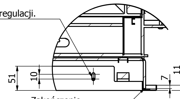
C (1:4)
